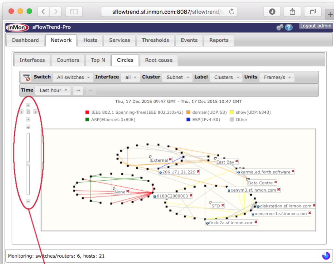
View controller
